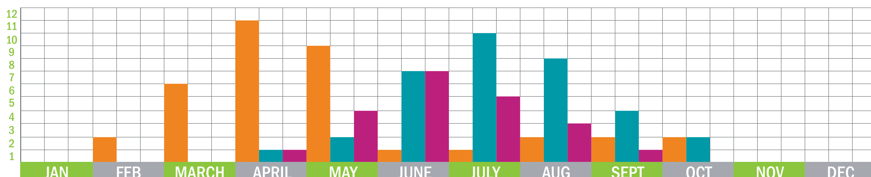
Number of seasonal allergens prominent in the Southeast by type and month.
