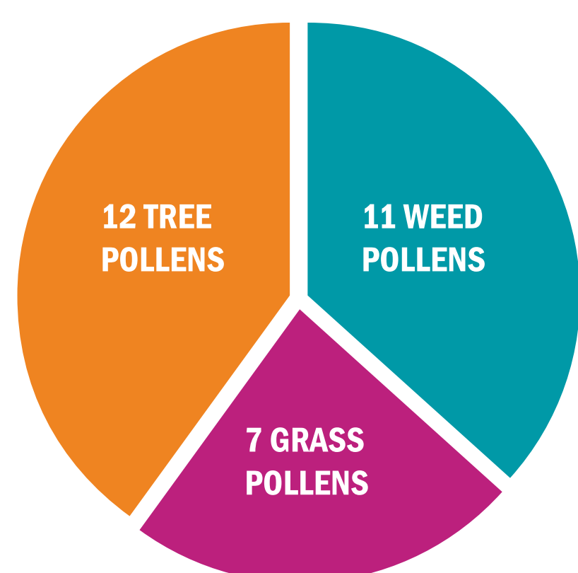
Number of seasonal allergens prominent in the Southeast by type.
